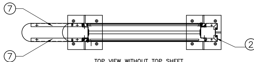
TOP VIEW WITHOUT TOP SHEET
